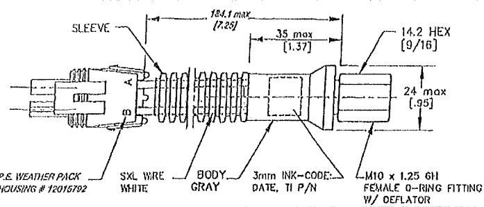
4108434 FREIGHTLINER HYDRAULIC FAN SWITCH
